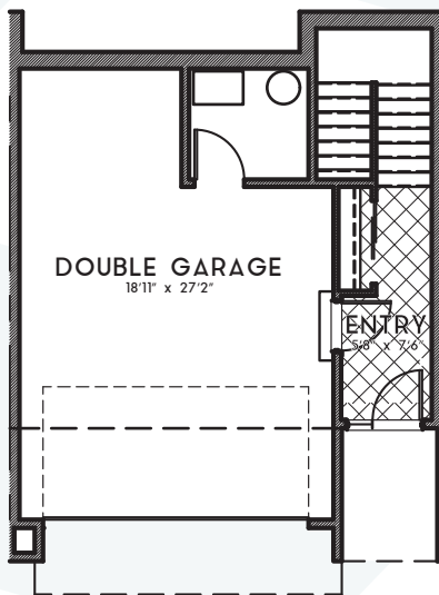
GROUND LEVEL 87 SQ.FT.
